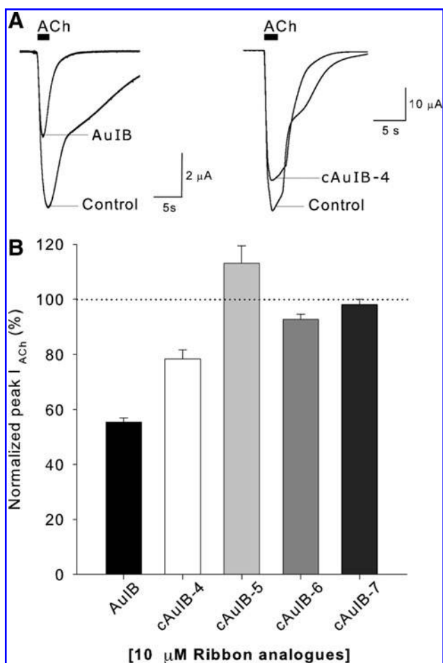
FIG. 8. Electrophysiological assays of ribbon AuIB analogs at \alpha\beta\gamma nAChRs expressed in Xenopus oocytes. (A) Representative ACh-evoked currents obtained in the absence (control) and presence of AuIB (ribbon) and cAuIB-4 (ribbon) (10 \mu M). (B) Bar graph of normalized peak current amplitudes showing comparison of inhibitory effects of AuIB [ribbon] analogs tested at 10 \mu M concentration.
